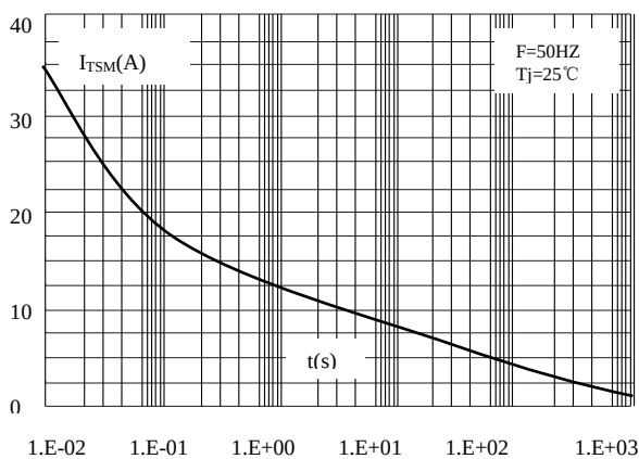
Fig.3 Non Repetitive Surge Peek On-State Current Versus Overload Duration
