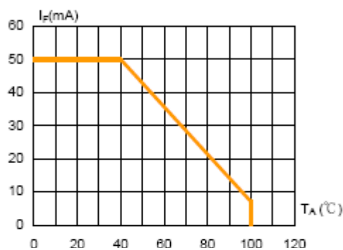
Fig. 4 Allowable Forward Current vs. Ambient Temperature
