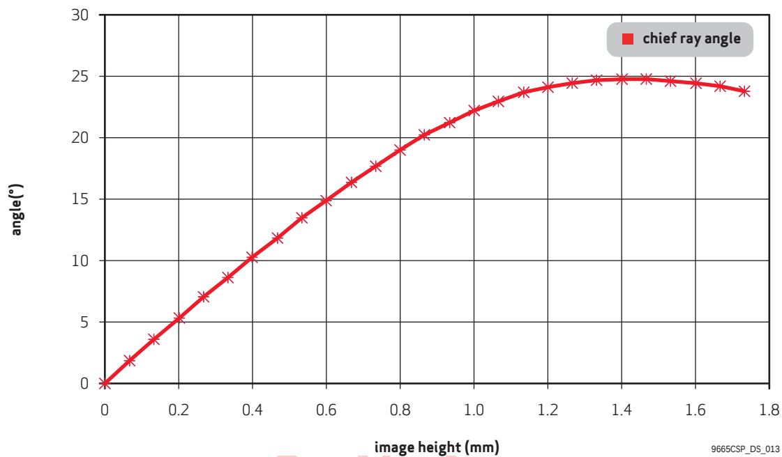
Figure 13 OV9665 Chief Ray Angle
