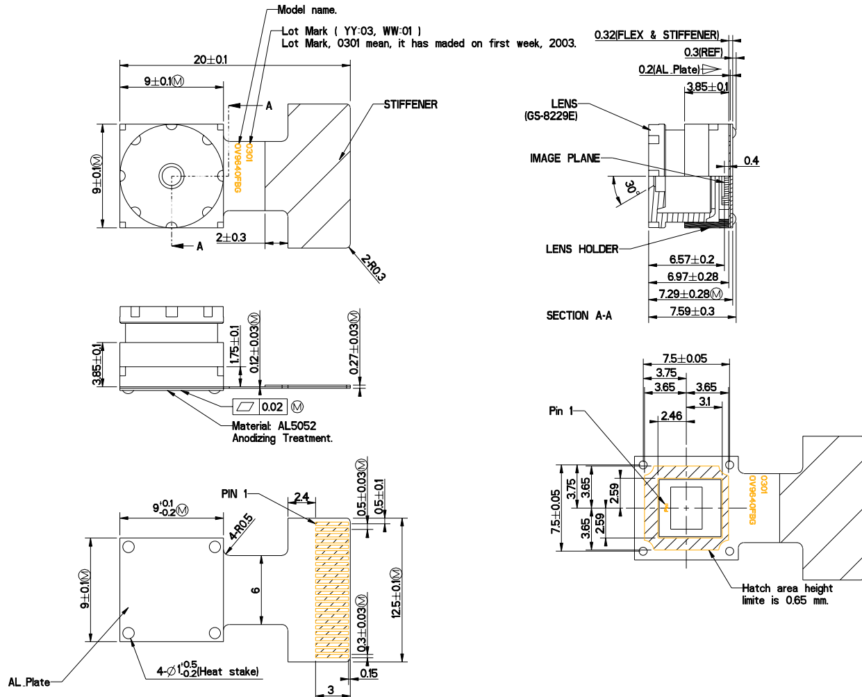
Figure 15 OV9640FBG Package Specifications
