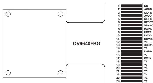
Figure 1 OV9640FBG Pin Diagram
