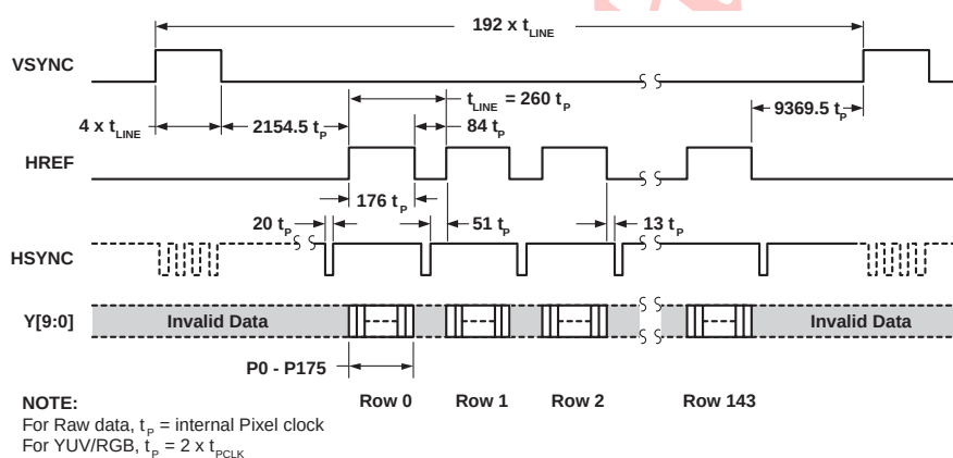
Figure 11 QCIF Frame Timing
