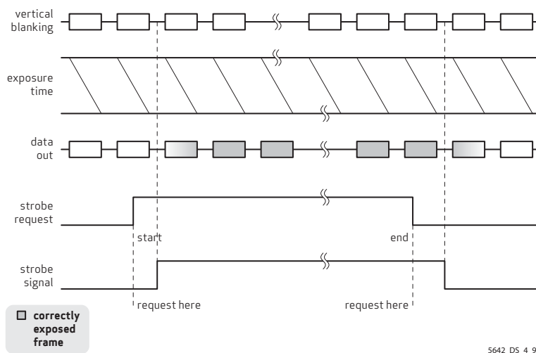
figure 4-9 LED 3 mode
