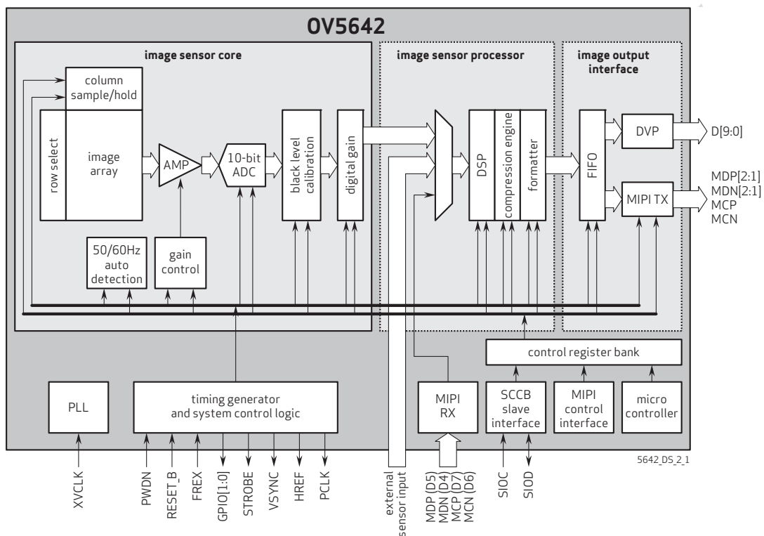
figure 2-1 OV5642 block diagram
