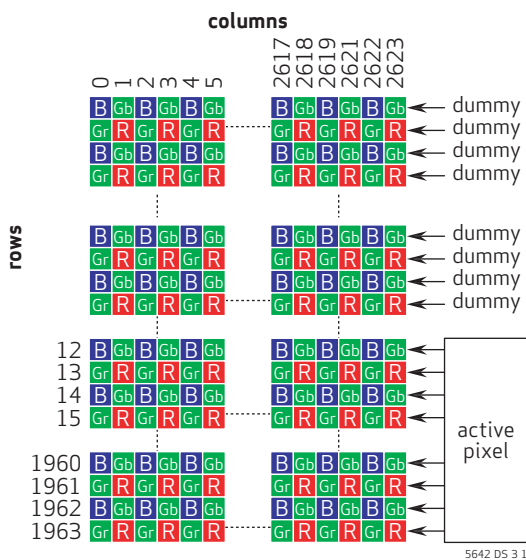
figure 3-1 sensor array region color filter layout
