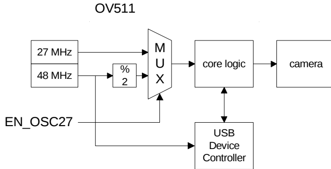
Figure 11. Clock Scheme of OV511
