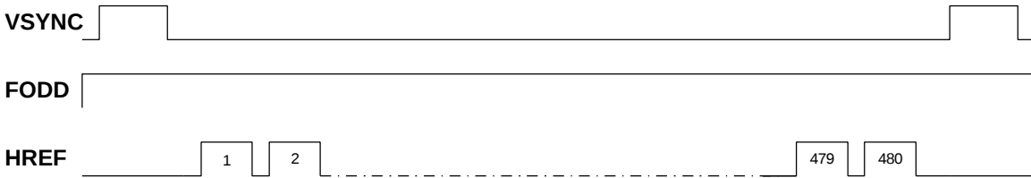
Figure 4. Camera Interface Vertical – Progressive Mode Timing Waveforms
