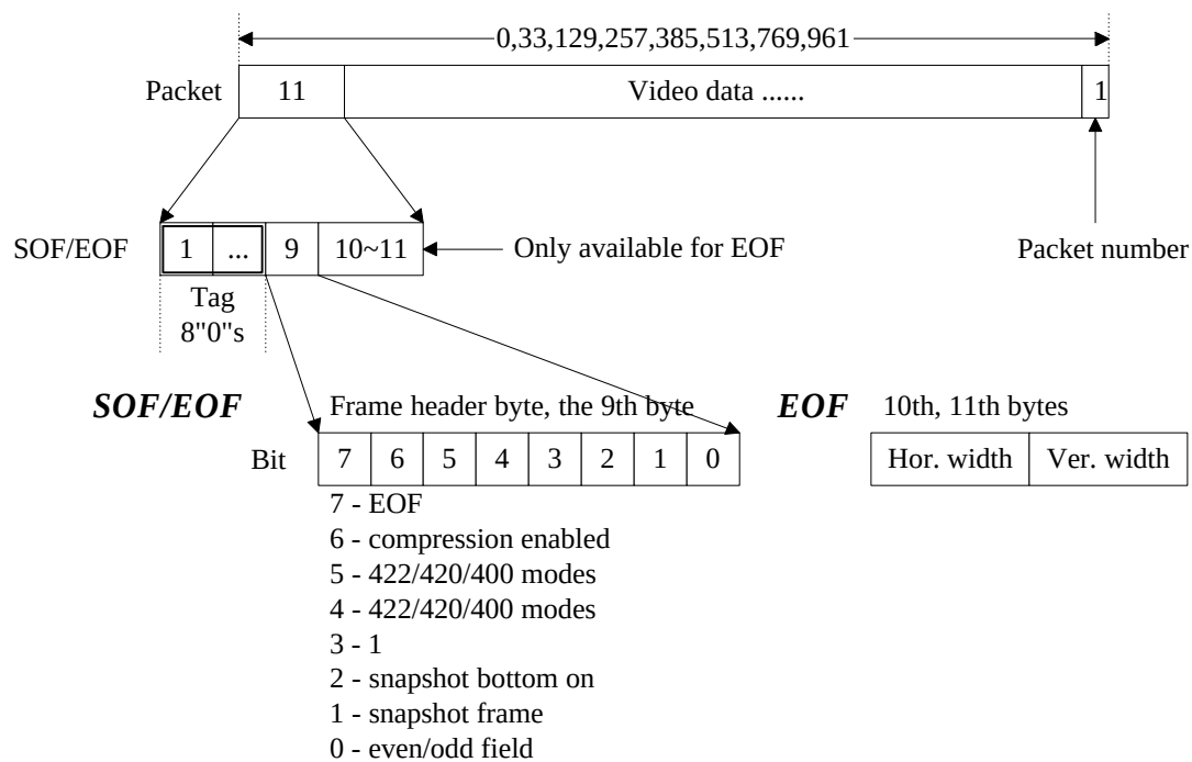
Figure 10. SOF/EOF Formats
