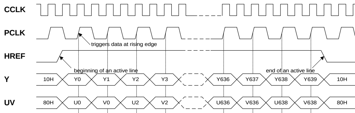
Figure 2. Camera Interface YUV - 4:2:2 - 16-bit Horizontal Timing Waveforms
