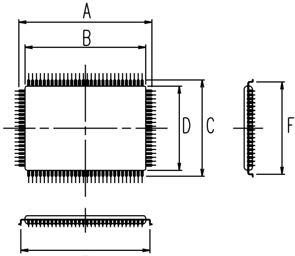
OTQ-100-0.65 (REFERENCE ONLY)
