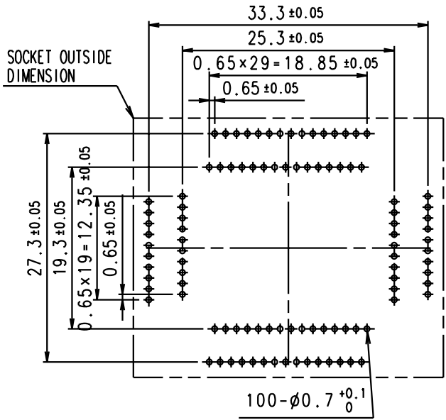
OTQ-100-0.65 (REFERENCE ONLY)
