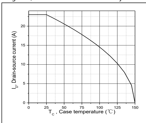
Figure 9, Drain current
