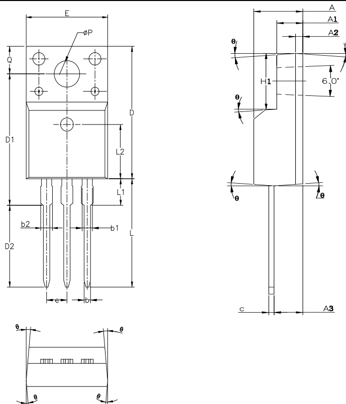
Figure1, TO220F package outline dimension
