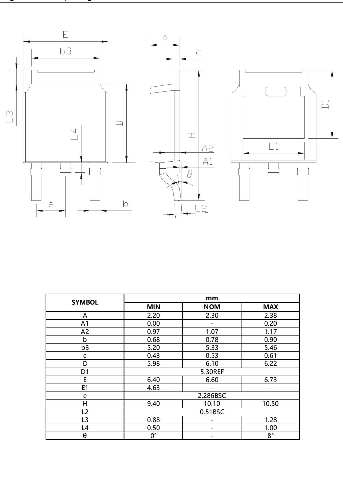
Figure2, TO252 package outline dimension
