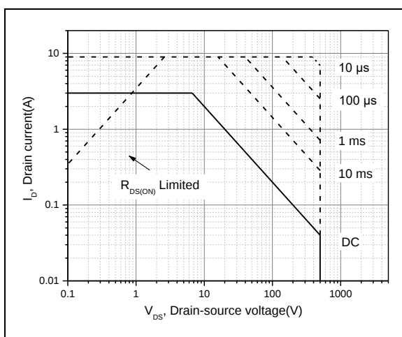
Figure 10, Safe operation area for TO251/TO252/TO220 T_C = 25\text{ }^{\circ}\text{C}
