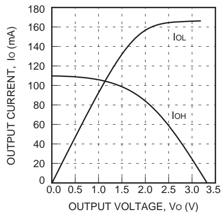
Figure 91. Fast ( T_J = 25^\circ\text{C} , V_{DD} = 3.3\text{ V} )
