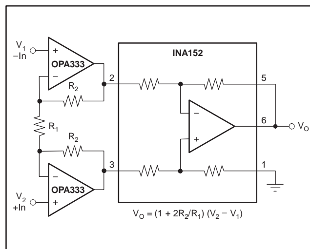
Figure 8. Precision Instrumentation Amplifier
