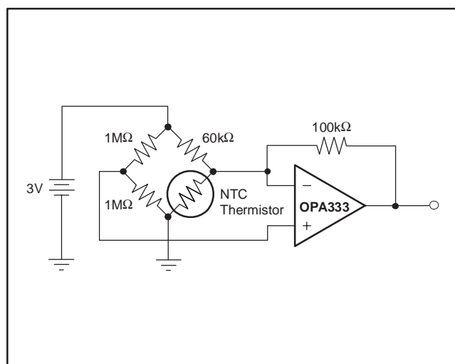
Figure 7. Thermistor Measurement
