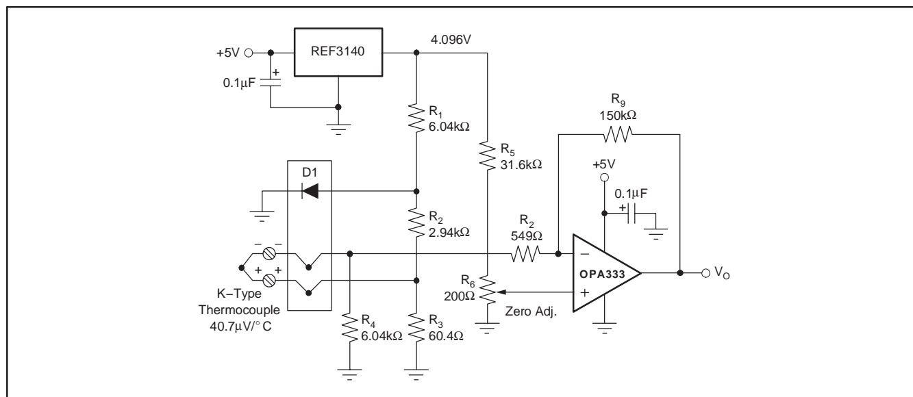
Figure 3. Temperature Measurement
