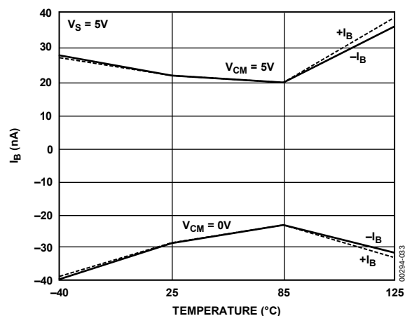
Figure 28. Input Bias Current vs. Temperature, V_S = 5V
