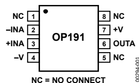
Figure 1. 8-Lead Narrow-Body SOIC
