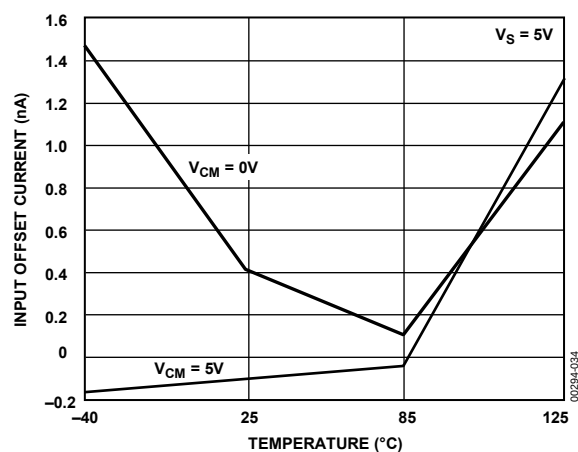
Figure 29. Input Offset Current vs. Temperature, V_S = 5V
