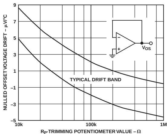
TPC 7. Nullled Offset Voltage Drift vs. Potentiometer Size
