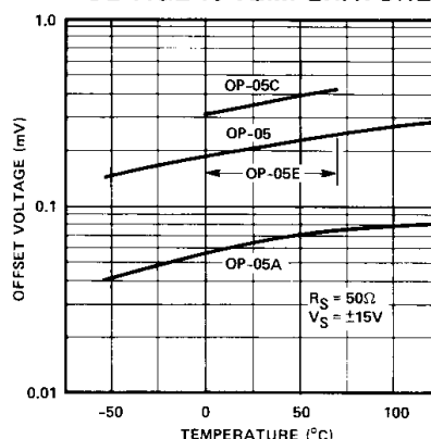
UNTRIMMED OFFSET VOLTAGE vs TEMPERATURE
