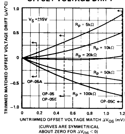
TRIMMED OFFSET VOLTAGE DRIFT
