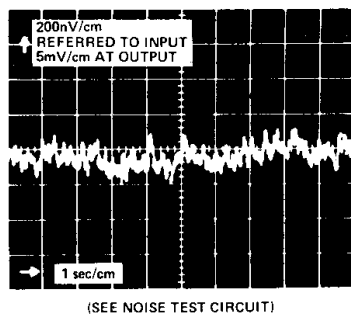
OP-05 LOW FREQUENCY NOISE
