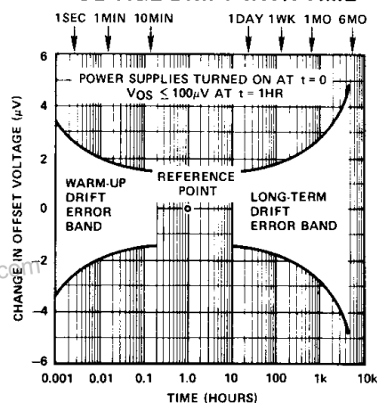
OFFSET VOLTAGE DRIFT WITH TIME
