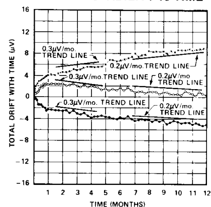
TYPICAL OFFSET VOLTAGE STABILITY vs TIME
