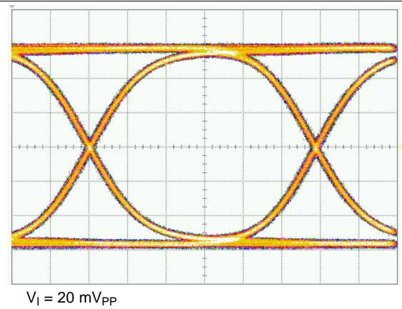
Figure 33. RX Output Eye-Diagram at 11.3 Gbps
