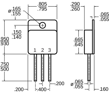
TO-267
