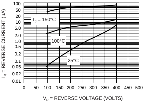
TYPICAL REVERSE CURRENT OM5240, 5241
