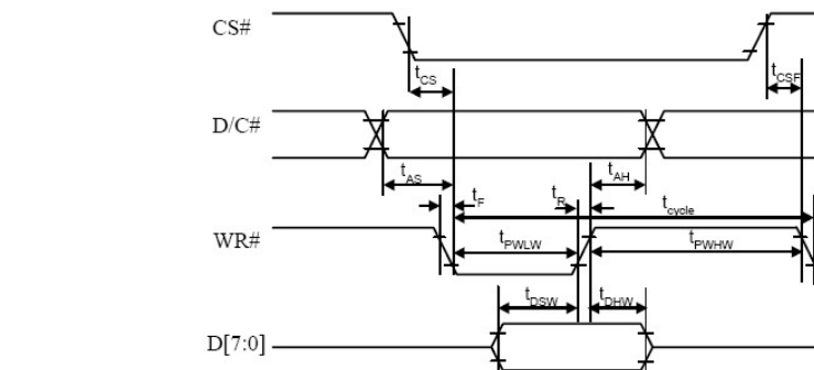
( Write Timing )
