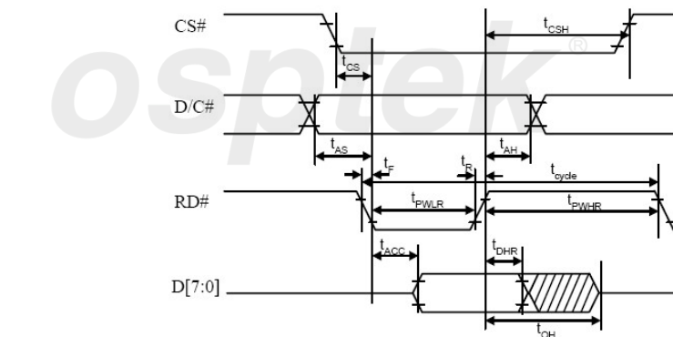
( Read Timing )
