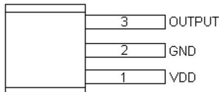
Figure 1, Pin Assignments of OCH1910
