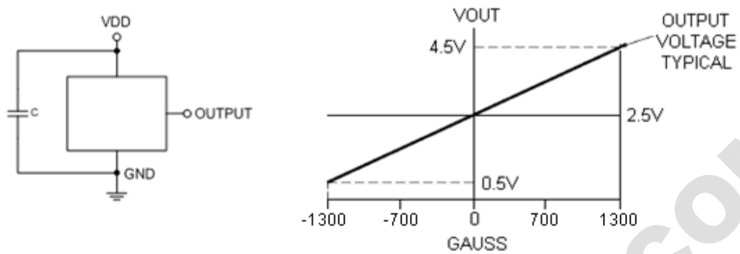
Figure 2, Typical Application of OCH1910
