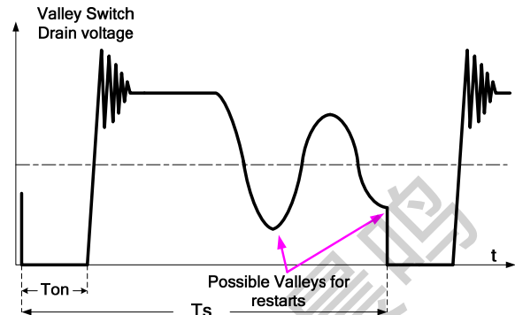
Fig3 Valley detection
