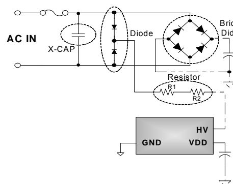
Fig9 X-CAP discharge circuit
