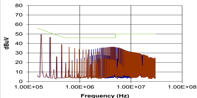
NXF1S0305MC (Average)
