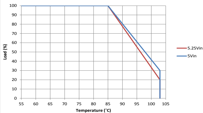
NXF1S0505MC
