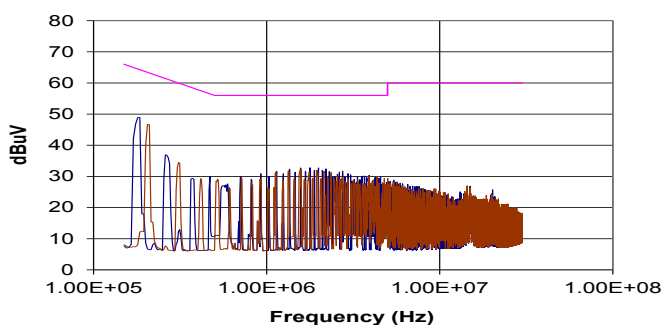
NXF1S0305MC (Quasi-Peak)
