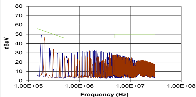
NXF1S0305MC (Average)
