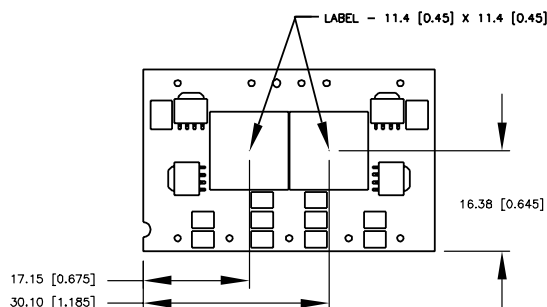
Figure 31. Pick and Place Location.
