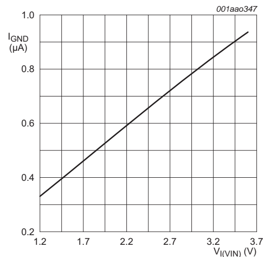
Fig 6. Waveform showing the ground current versus input voltage on pin VIN
