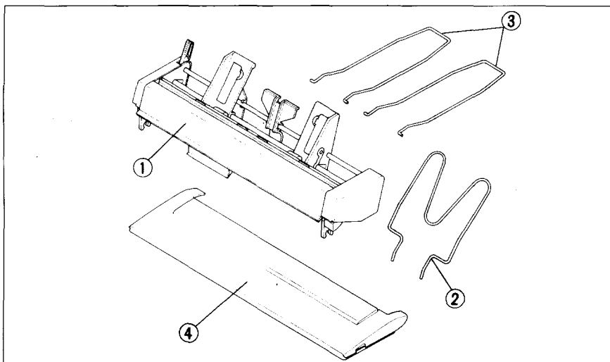
Figure 7-1. Check to make sure you have all five items: 1) Sheet Feeder, 2) Hopper attachment, 3) Stacker attachment, and 4) Printer cover, and 5) ASF User's manual.
