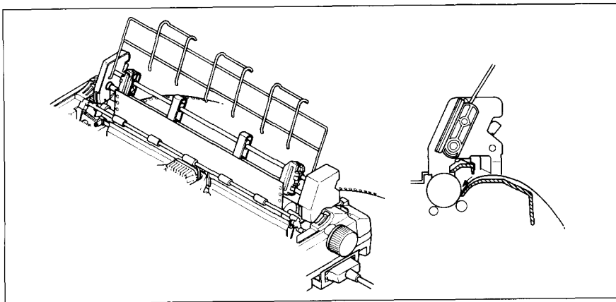
Figure 7-13. Insert the paper from the entry slot for cut-sheet forms.
