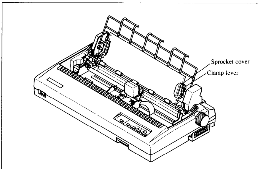
Figure 1-16. Thread the fanfold paper over the sprockets from the entry slot of the printer.
