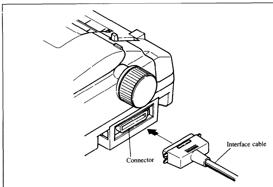
Figure 1-8. Connecting the interface cable
