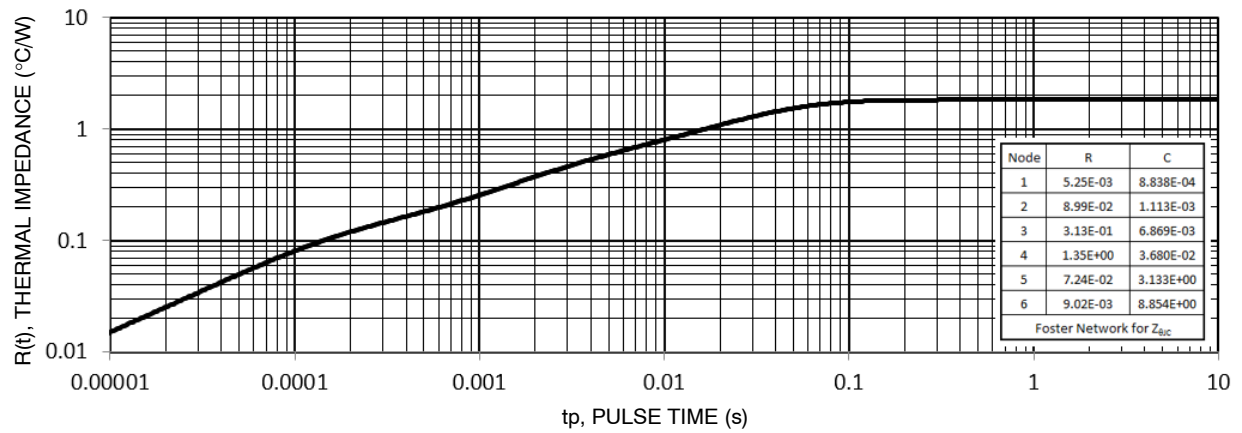
Figure 13. Thermal Response
