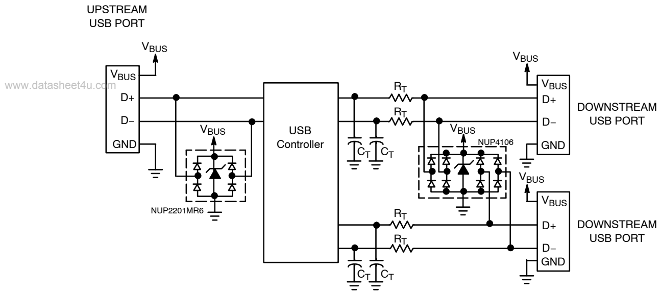
Figure 10. ESD Protection for USB Port
