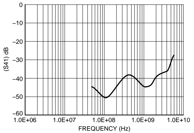
Figure 2. Analog Crosstalk
