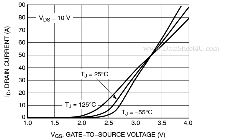
Figure 2. Transfer Characteristics
