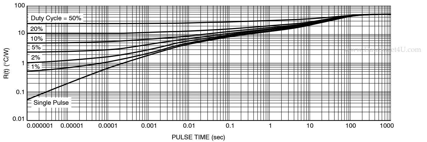
Figure 13. Thermal Response
