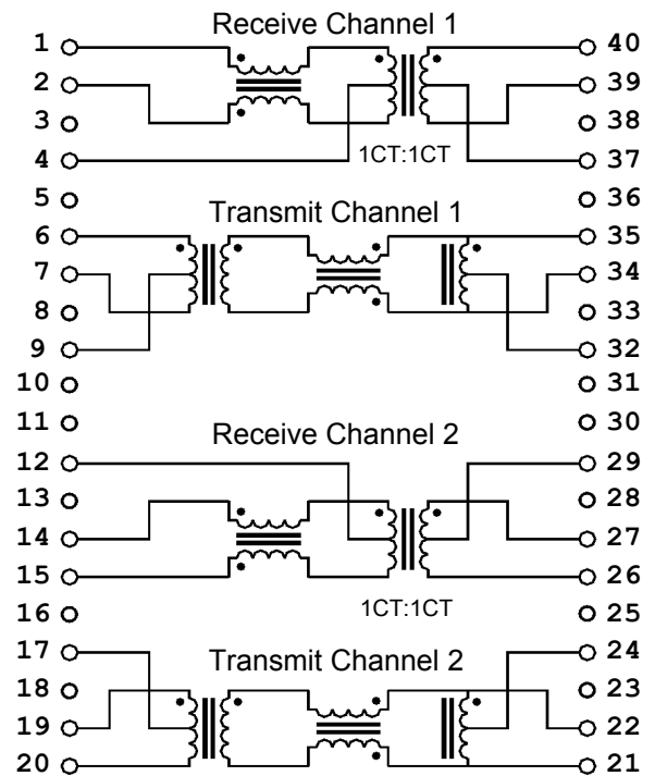
Circuit 2
