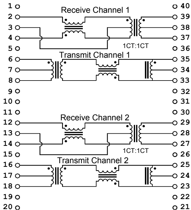
Circuit 3
