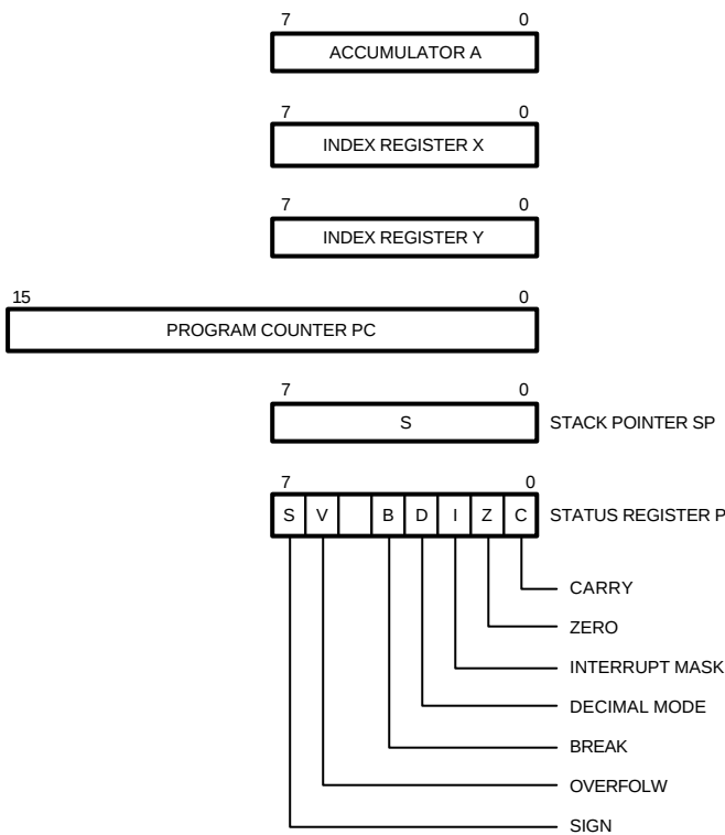
Figure 1. 6502 CPU Registers and Status Flags
