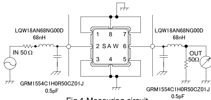
Fig.1 Measuring circuit
