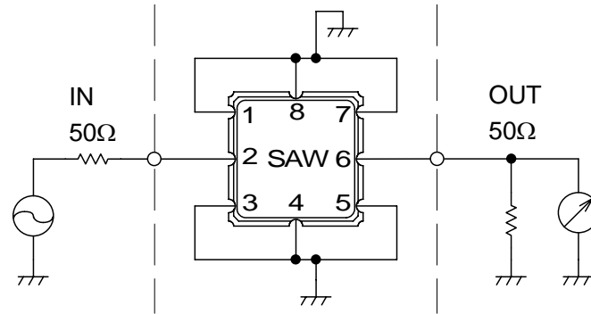
Fig.1 Measuring circuit
