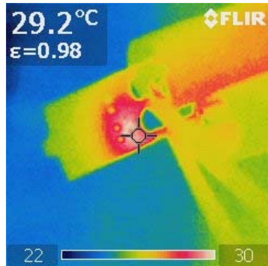
Figure 9. Case Temperature of NSR05F40NXT5G in Operation at 25°C, 150 mA 34 V Output
