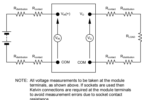
Figure 45. Output Voltage and Efficiency Test Setup.
