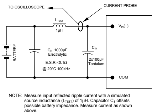
Figure 43. Input Reflected Ripple Current Test Setup.
