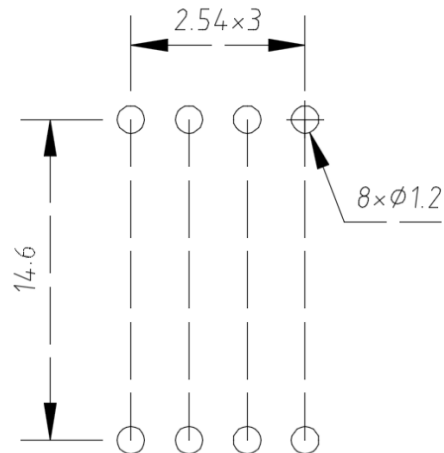
Figure 8.2 Footprint mm
