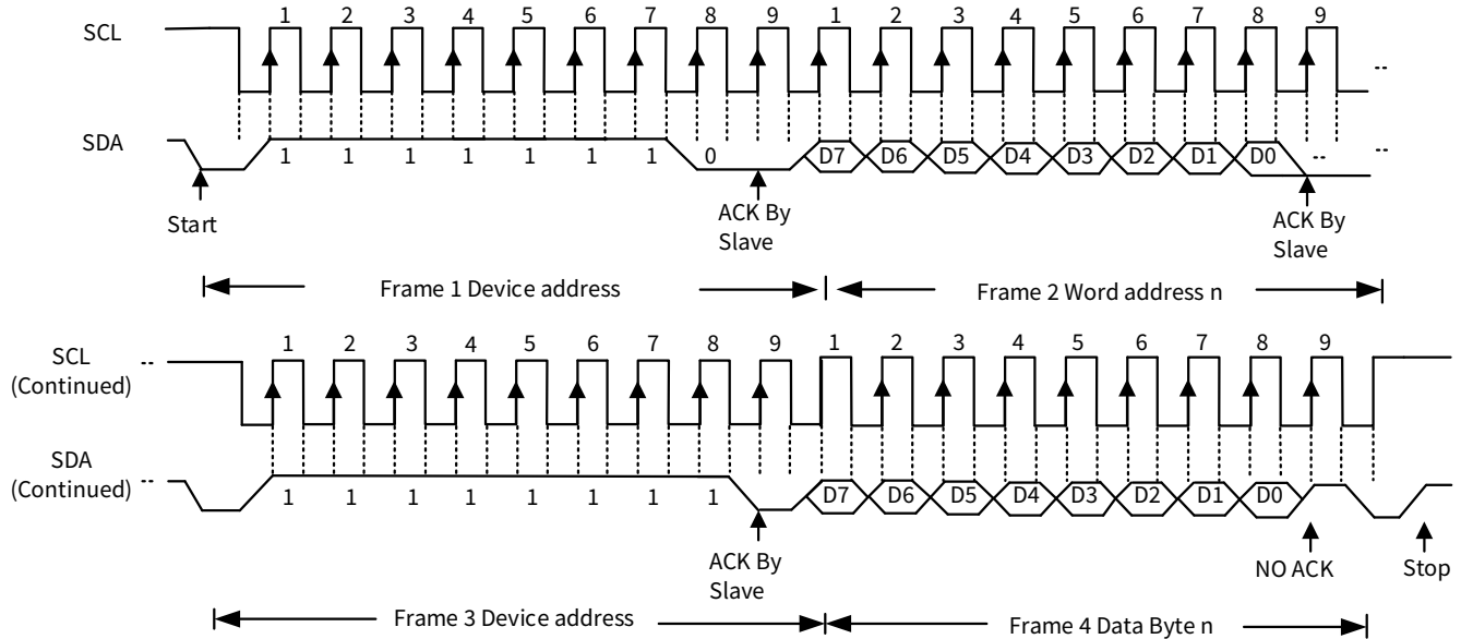
Figure 6.6 I²C Read Byte
