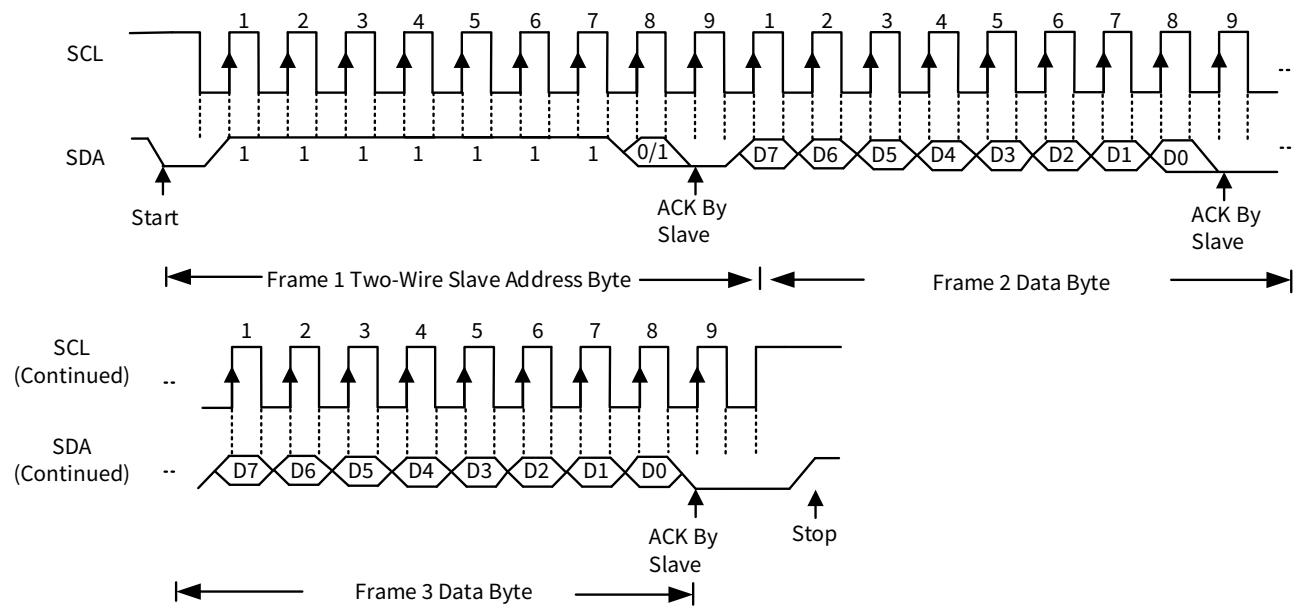
Figure 6.4 I²C Protocol
