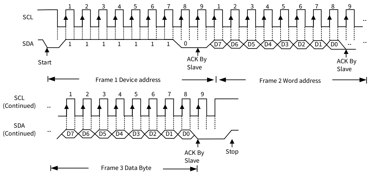
Figure 6.5 I²C Write Byte
