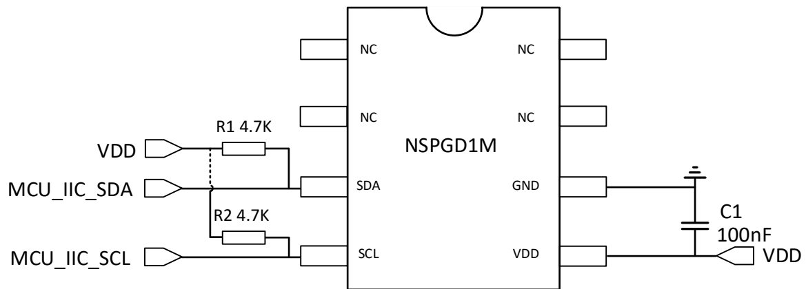
Figure 7.3 I²C Output Application Circuit
