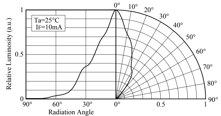
■ Directivity (NSPE520S)
