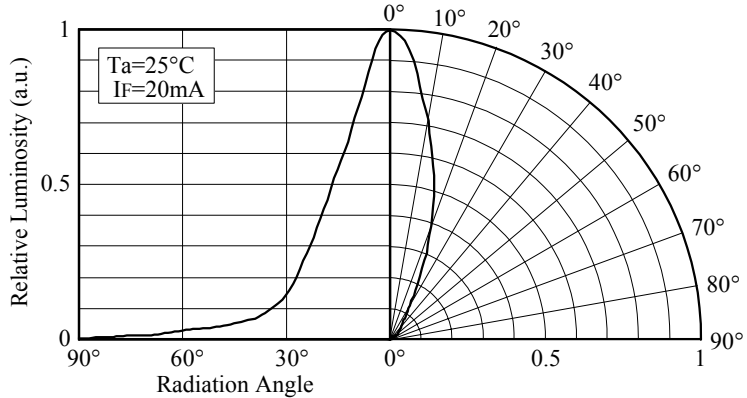
■ Directivity (NSPB310A)
