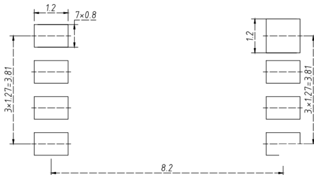
Fig 7.2 Footprint mm
