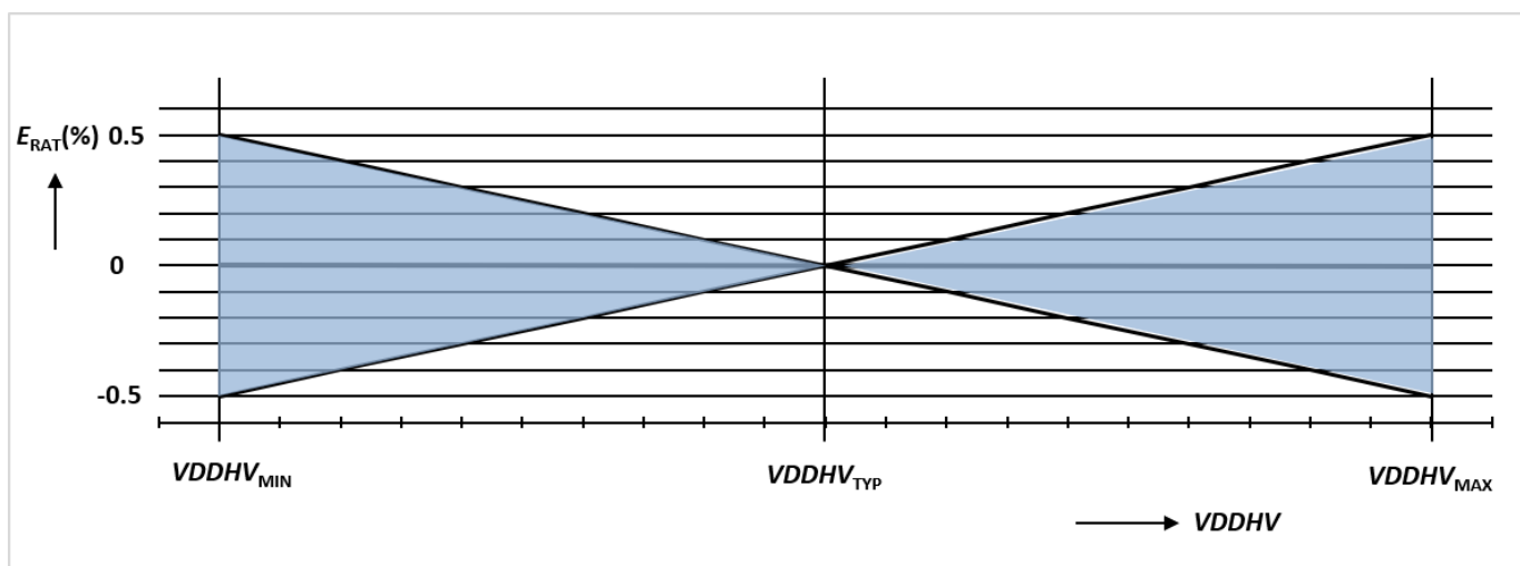
Fig 6.3 Ratiometric Error
