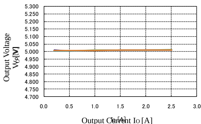
NR116K Load Reg. V_O = 3.3V L = 10\mu H T_a = 25^\circ C
