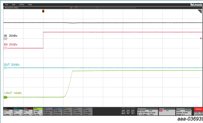
Fig. 7. Enable to short
