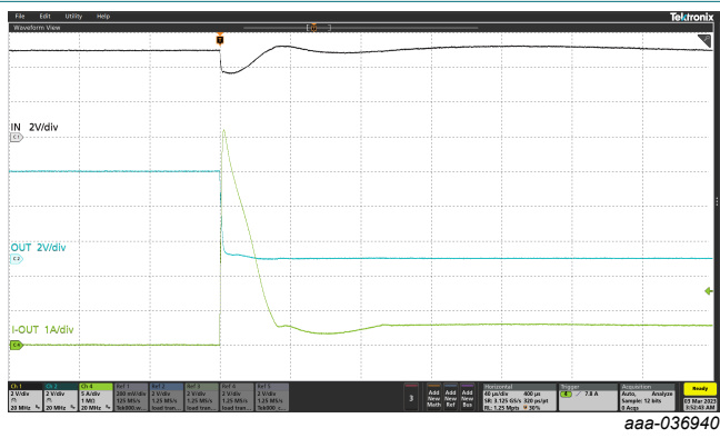
Fig. 8. Hard short
