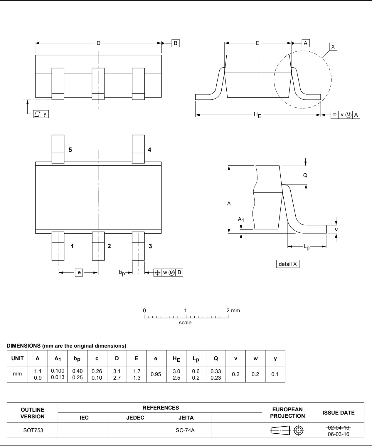
Fig. 21. Package outline SOT753 (SC-74A)
