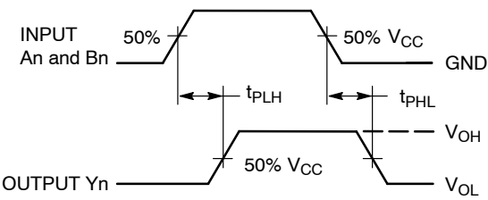
Figure 3. Switching Waveform
