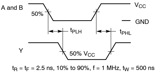
Figure 3. Switching Waveforms
