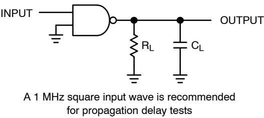
Figure 4. Test Circuit
