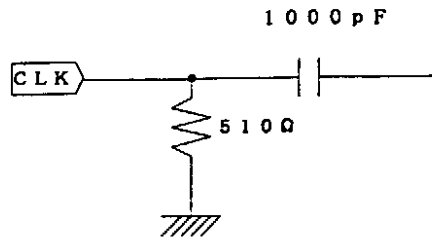
CLK input equivalent circuit
