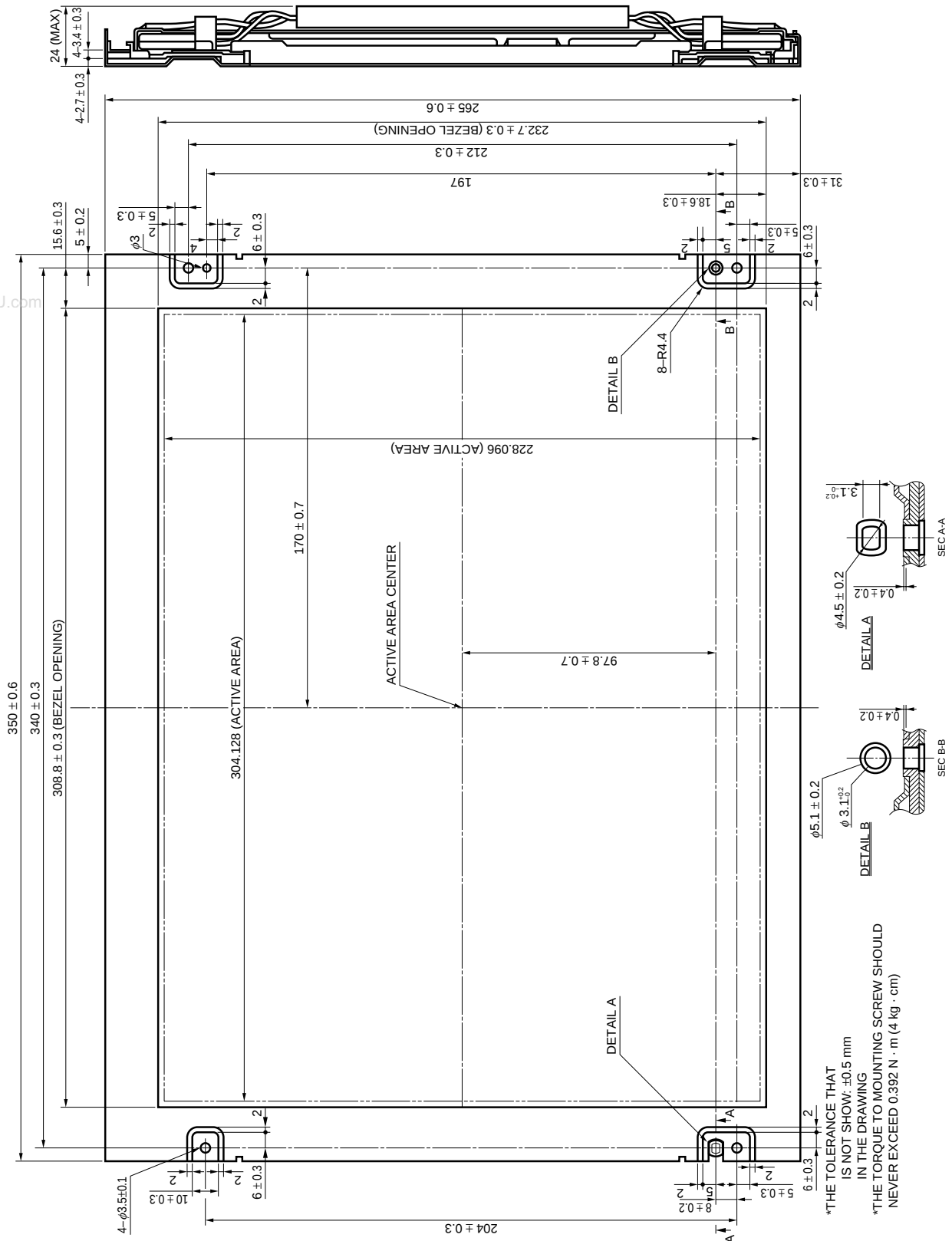
OUTLINE DRAWINGS: FRONT VIEW (Unit: mm)
