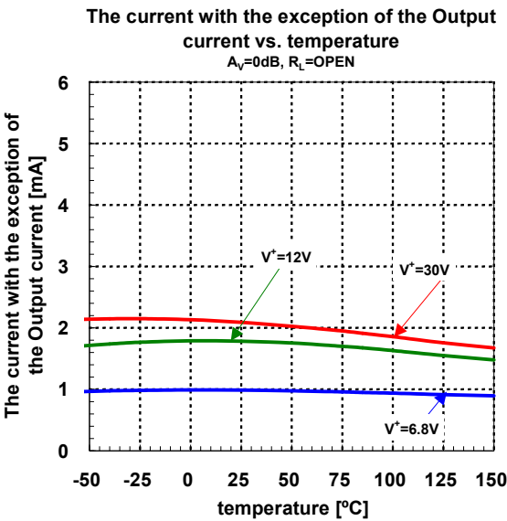
Fig1.12 the current with the exception of the Output current vs. temperature
