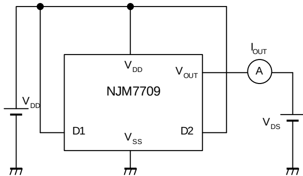
● Nch Output Current TEST CIRCUIT
