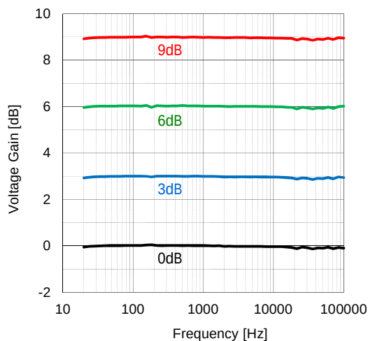
Voltage Gain Output vs Frequency V^+=9V , T_a=25^\circ C , V_{in}=0.1V_{rms} , Bandpass
